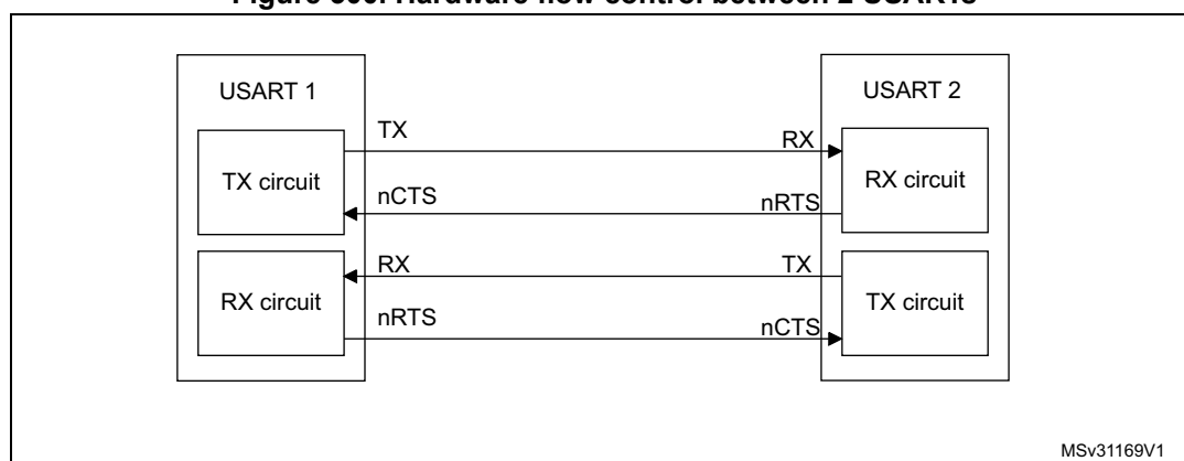
Figure 300. Hardware flow control between 2 USARTs
