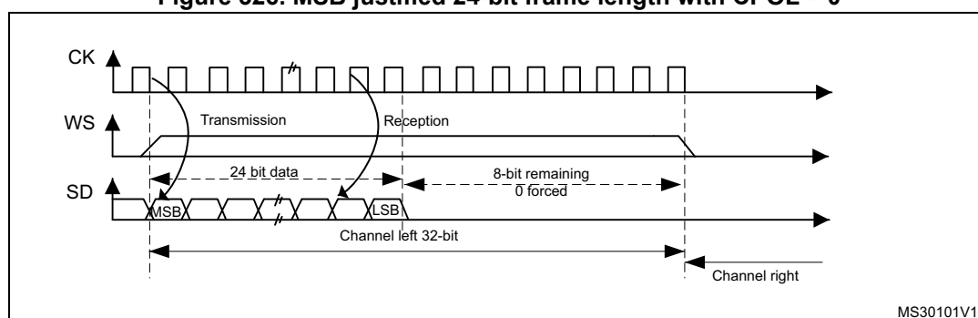
Figure 326. MSB justified 24-bit frame length with CPOL = 0
