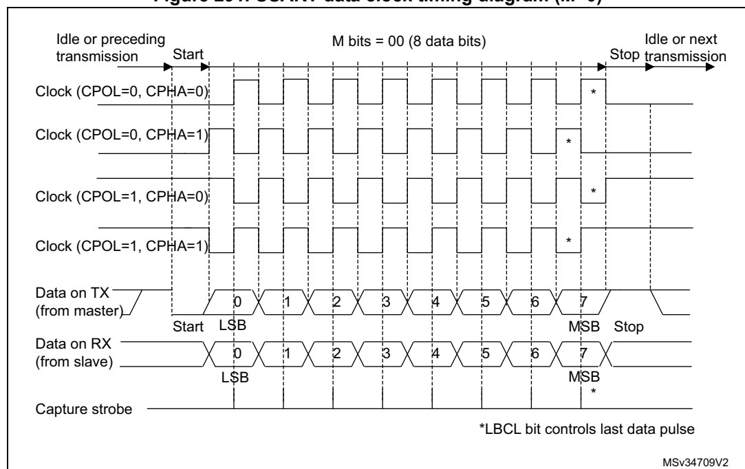
Figure 291. USART data clock timing diagram (M=0)
