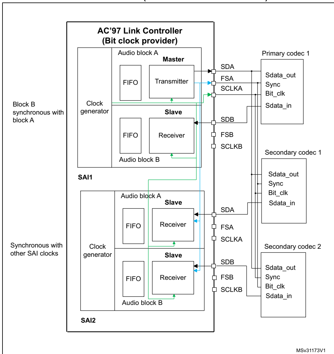
Figure 362. Example of typical AC'97 configuration on devices featuring at least 2 embedded SAIs (three external AC'97 decoders)
