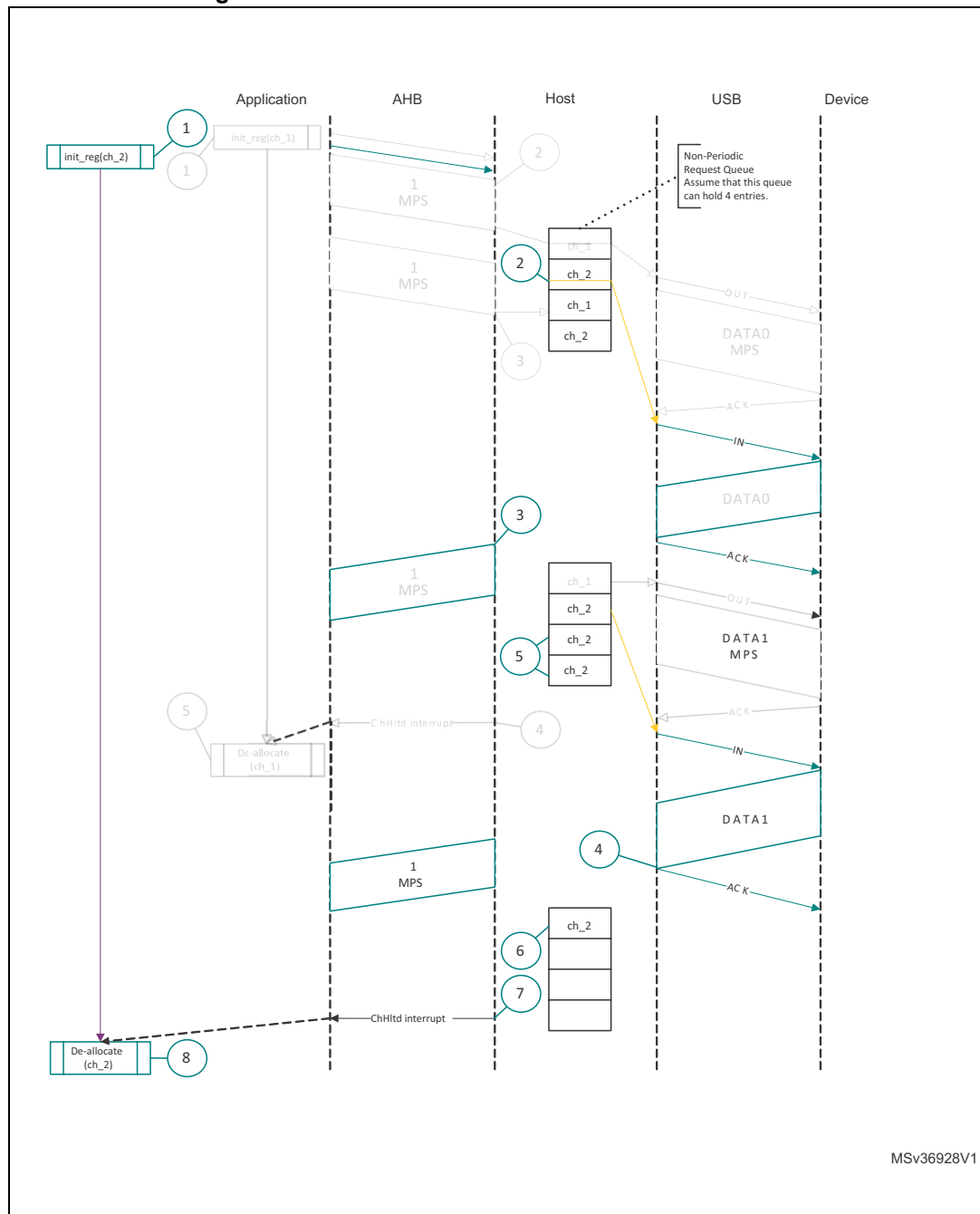
Figure 419. Normal bulk/control IN transaction - DMA
