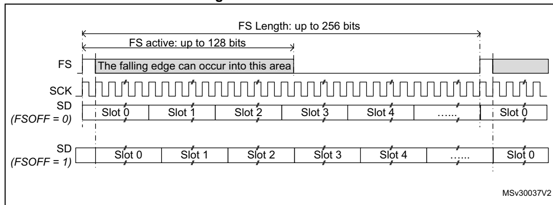
Figure 355. Audio frame
