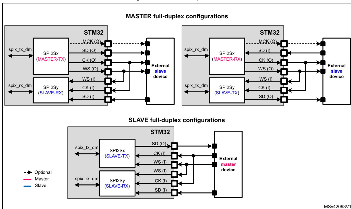
Figure 318. Full-duplex communication
