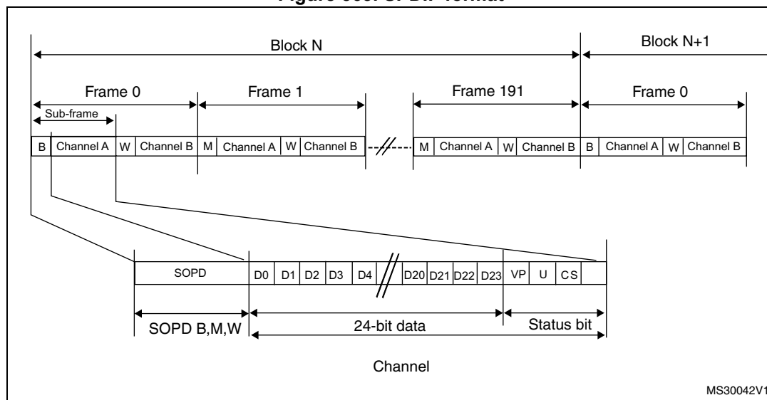
Figure 363. SPDIF format
