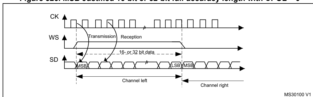
Figure 325. MSB Justified 16-bit or 32-bit full-accuracy length with CPOL = 0
