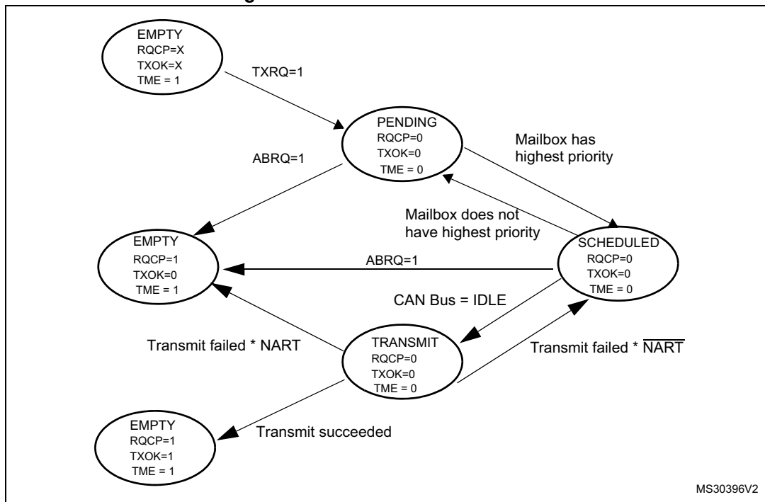
Figure 390. Transmit mailbox states
