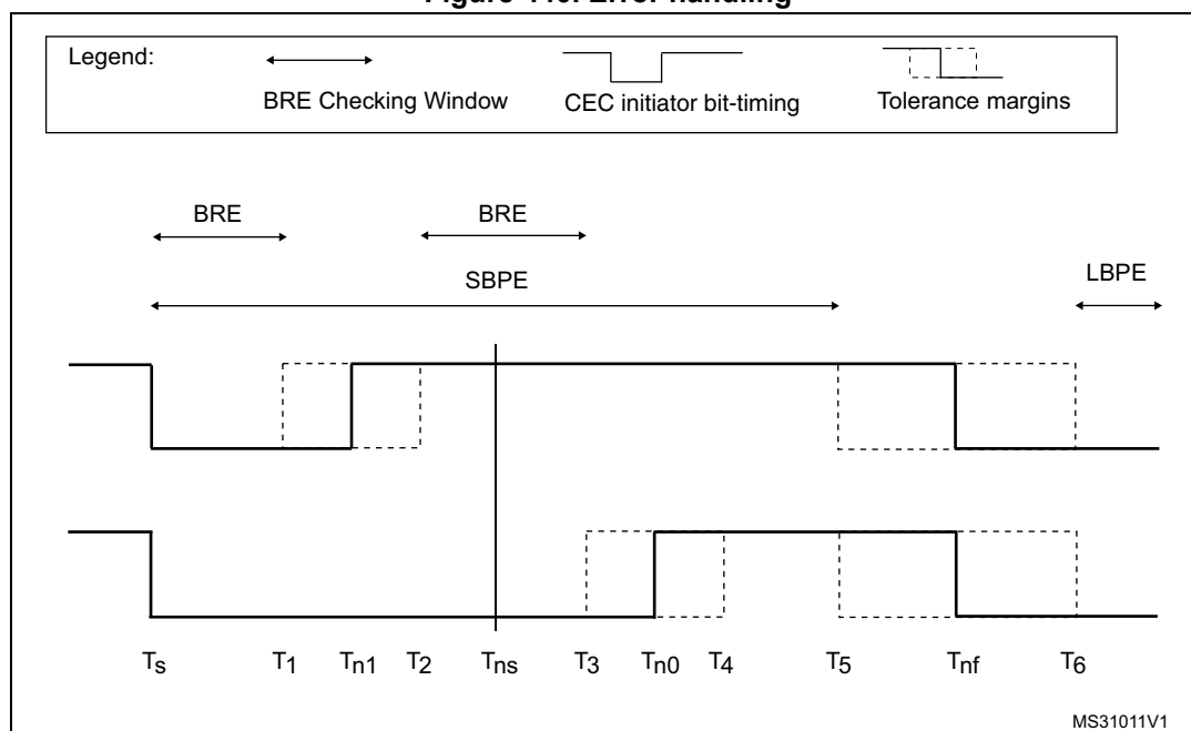
Figure 440. Error handling
